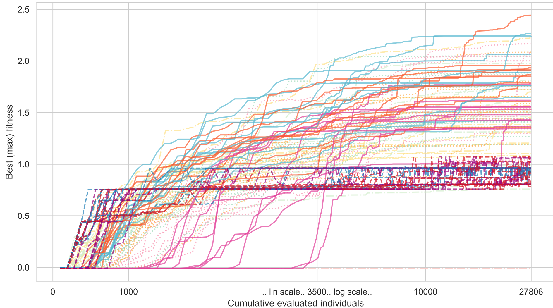
Best result vs evaluations (colored by enc)
